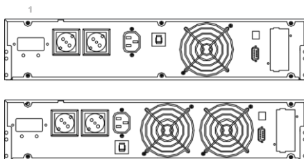
DSP Rack 1500 / 2500 / 3500
